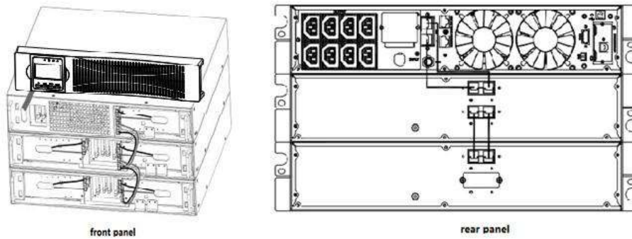
.Figure3 Typical EBP Installation
