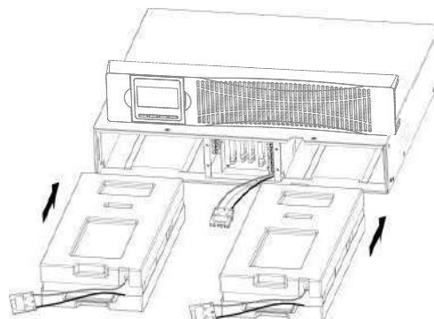
Fig.5 Installation for battery pack
